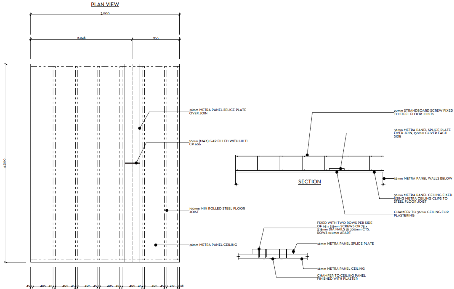
Figure 1: Client Supplied Plan and Section View of the Floor/Ceiling Assembly
