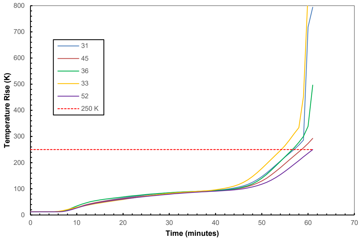
Figure 10: Incipient Spread of Fire Maximum Temperature Rise
